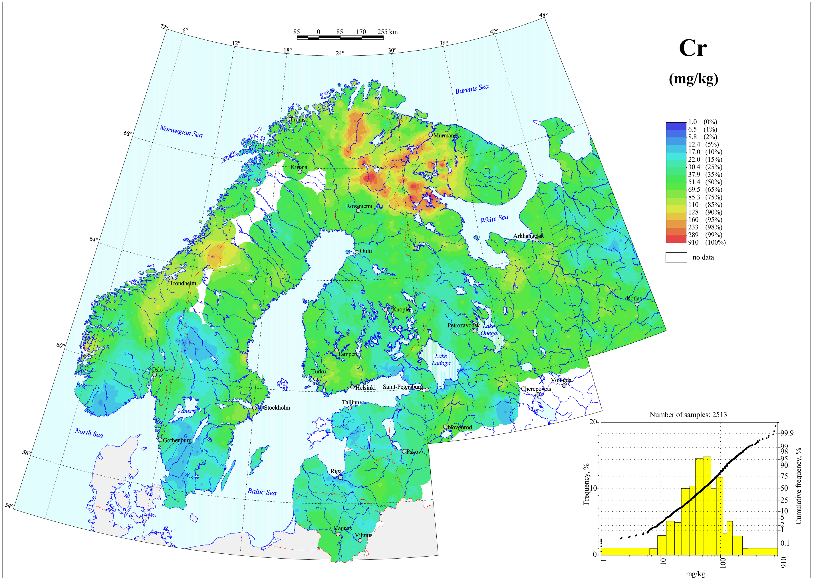
Chromium in C-horizon, Grain Size <2 mm, Total Content
